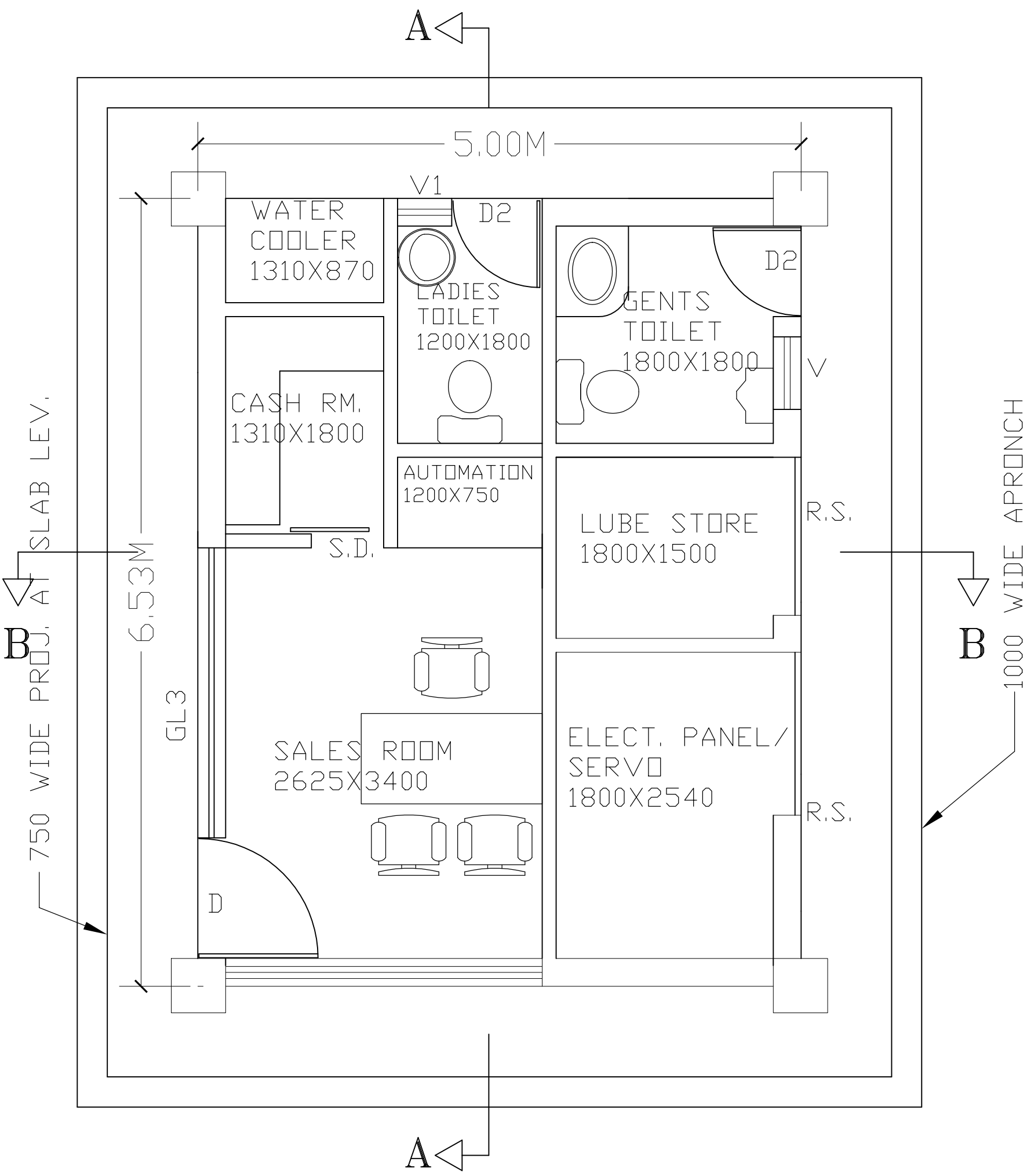
GROUND FLOOR LAYOUT PLAN
