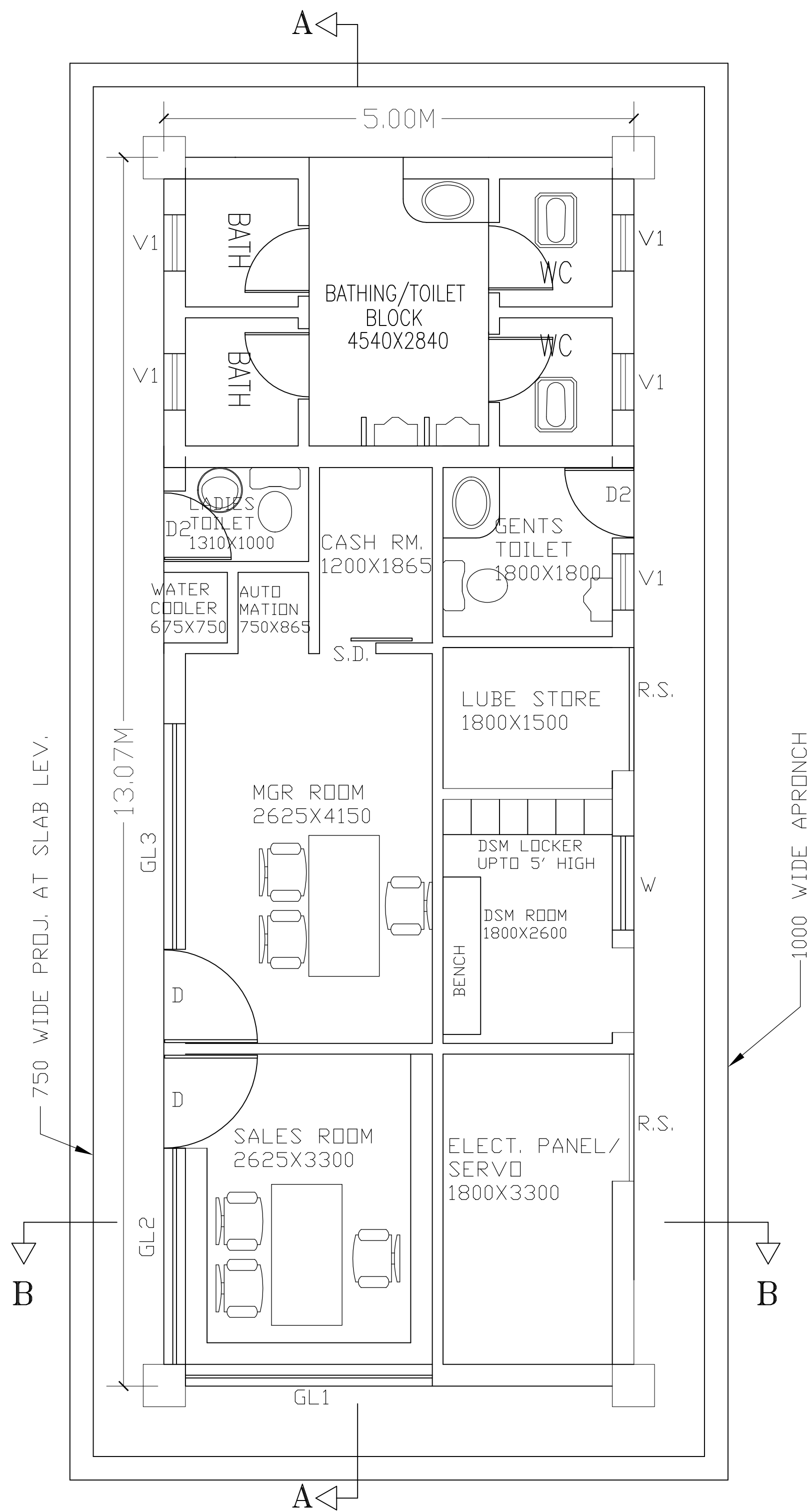
GROUND FLOOR LAYOUT PLAN
