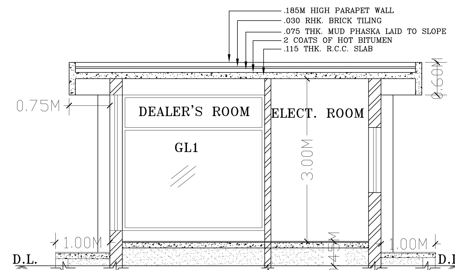
SECTION B-B
