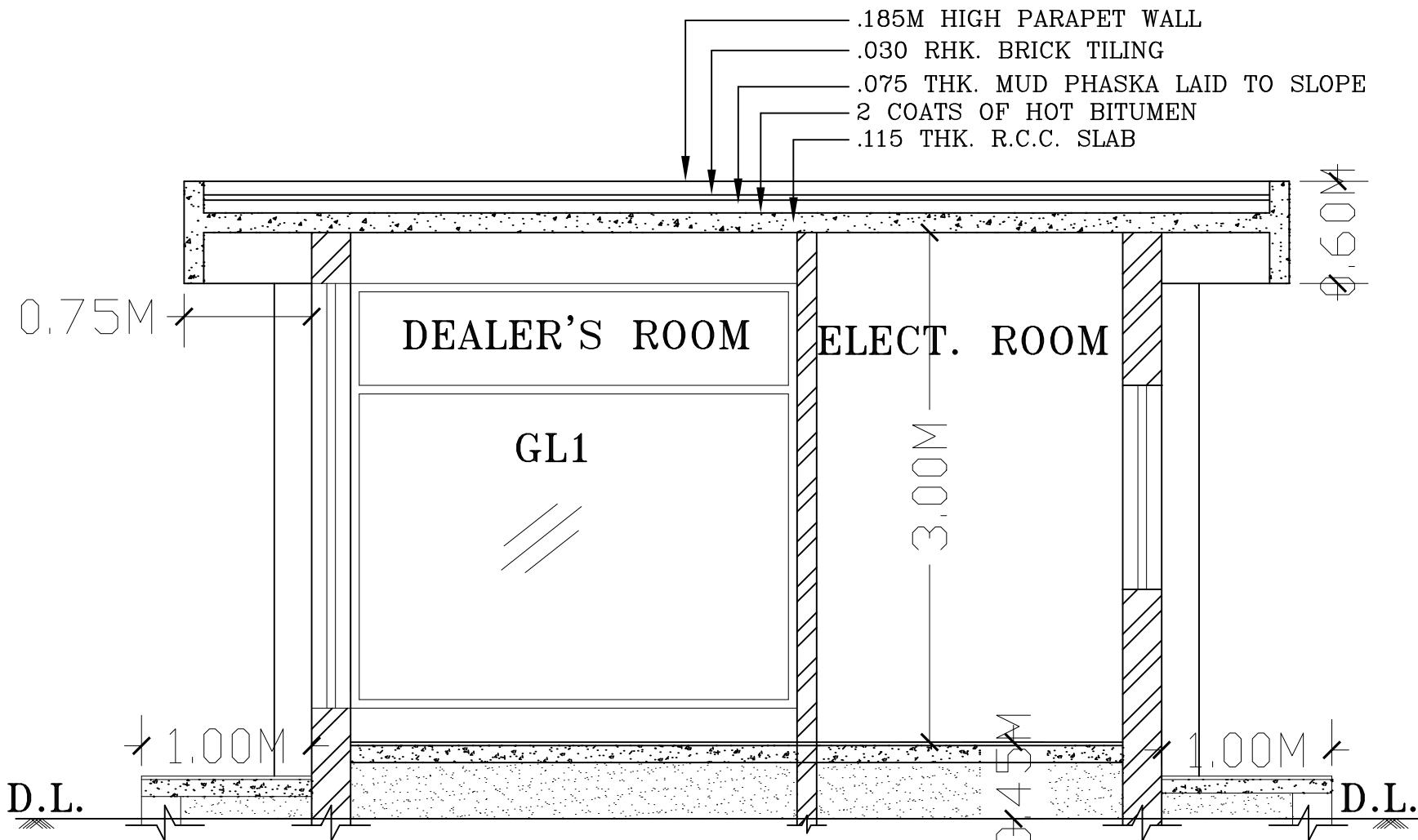
SECTION B-B
