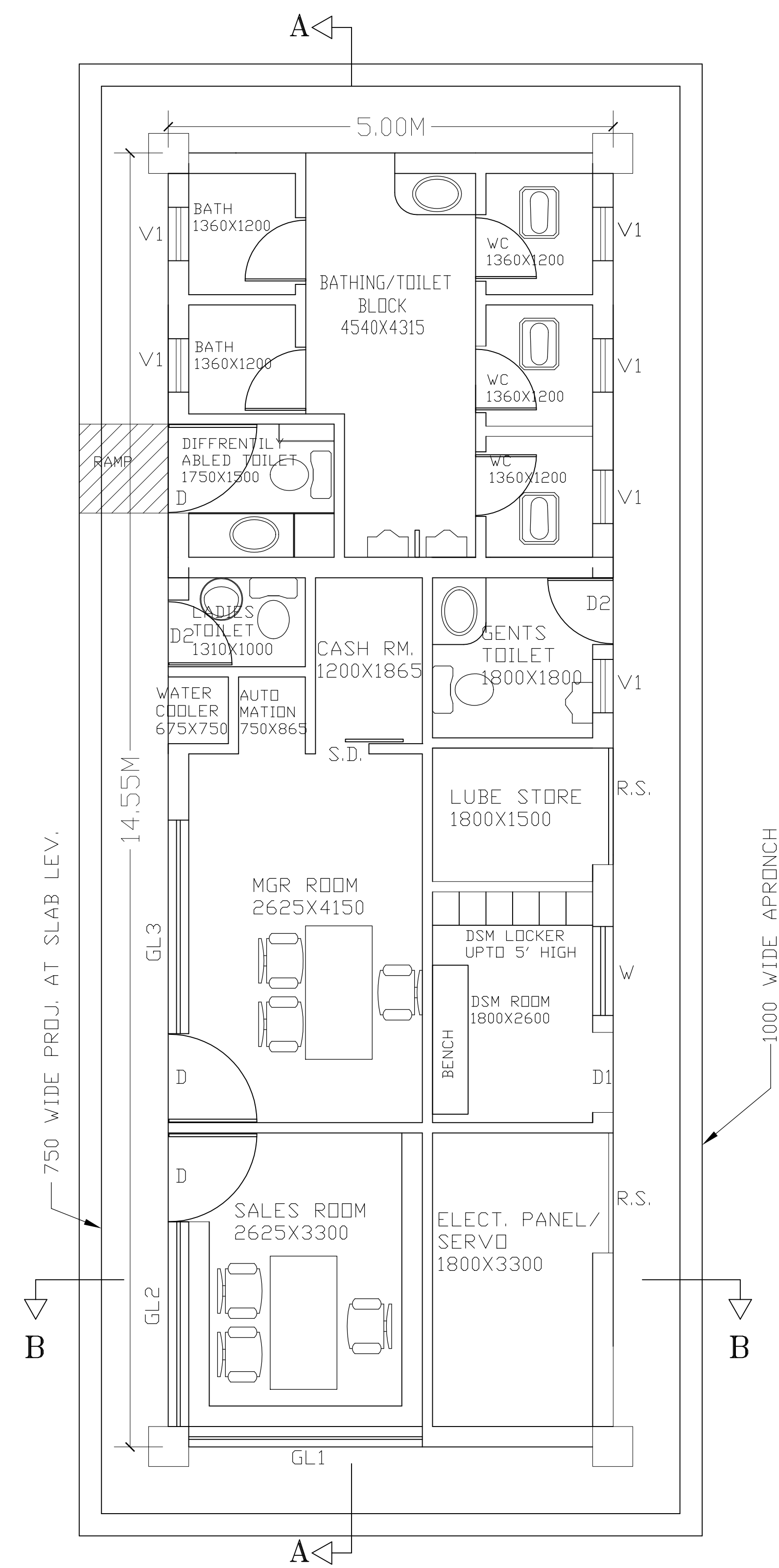
GROUND FLOOR LAYOUT PLAN
