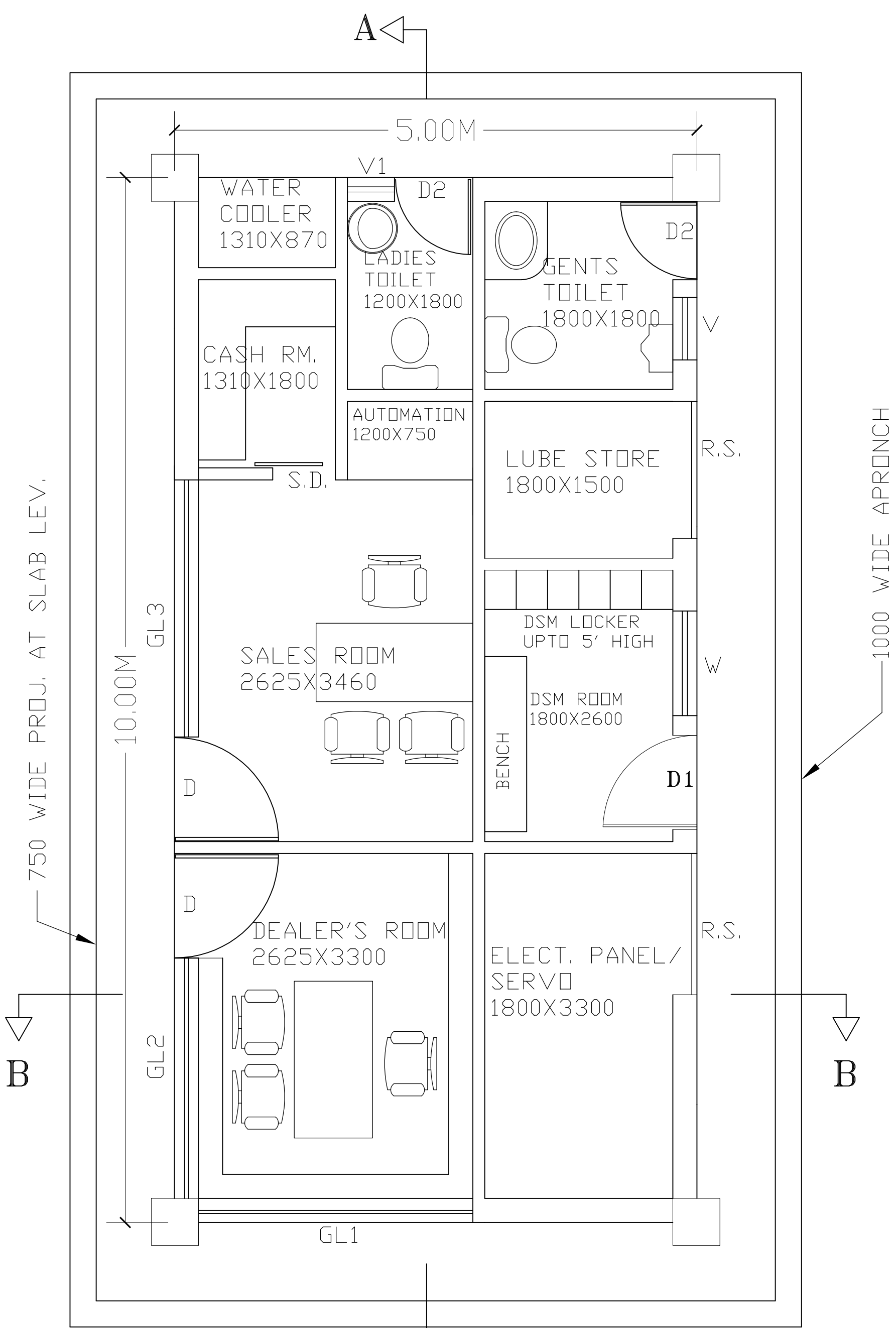
GROUND FLOOR LAYOUT PLAN
