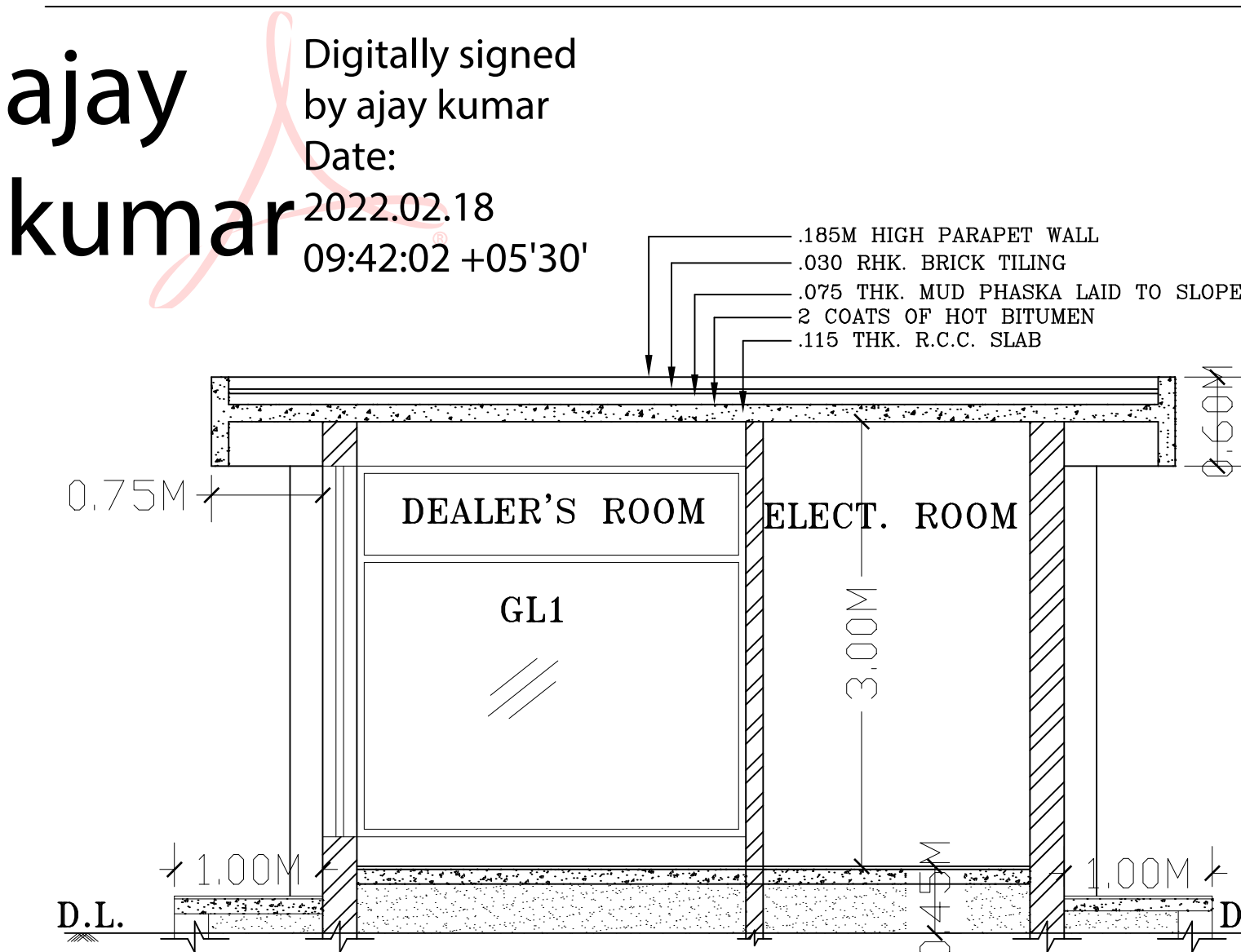
SECTION B-B
